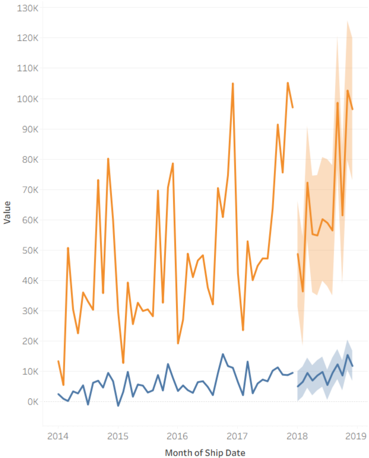
Line chart
