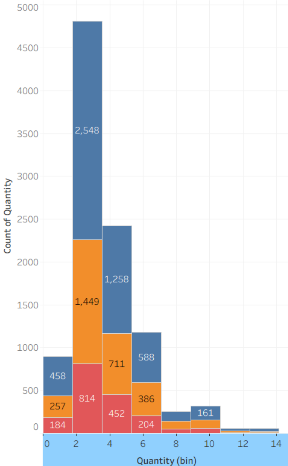
Histogram
